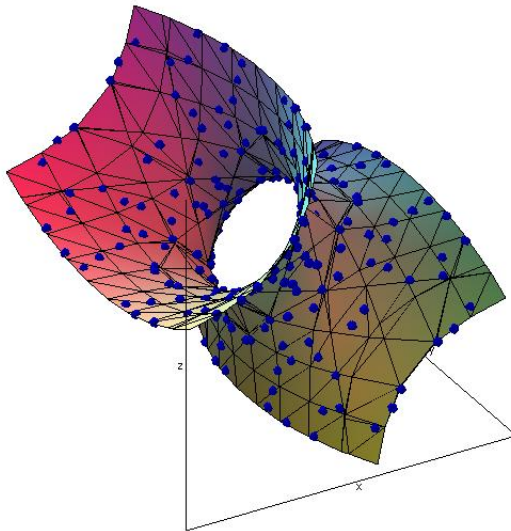
FIGURE 1. The distribution of 377^{-1/2}\mathbf{R}_{\text{disc}}(377) viewed on the one-sheeted hyperboloid, note that h(377) = 1 .
