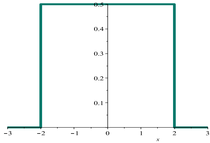
Solution at time t=1
