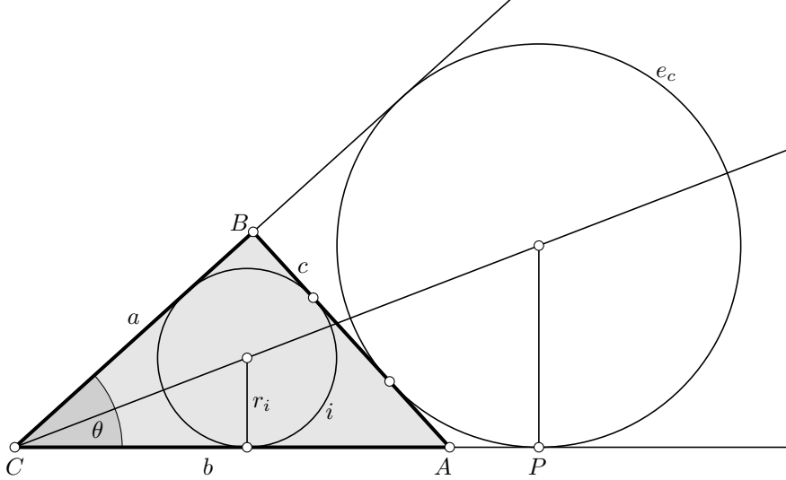
Figure 1: Triangle given by angle \theta , perimeter p = 2|CP| and area A = \frac{p}{2}r_i .
