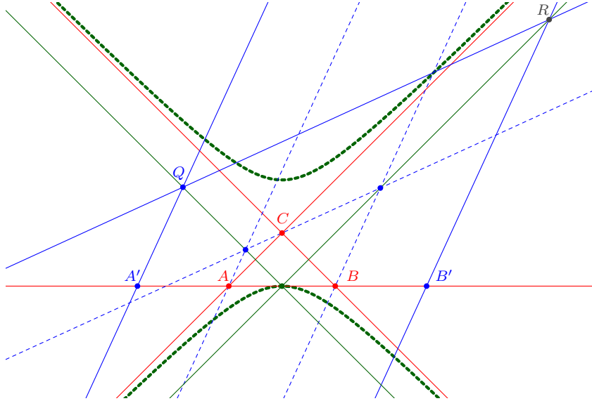
Figure 5: The situation when A \neq A' .
