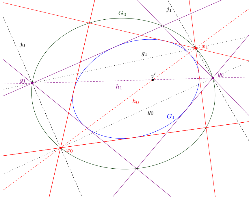
Figure 12: The two conics with the two Poncelet quadrilateral.
