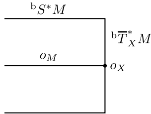
FIGURE 2. The radially compactified cotangent bundle {}^b\overline{T}^* M near {}^b\overline{T}_X^* M ; the cosphere bundle {}^bS^* M , viewed as the boundary at fiber infinity of {}^b\overline{T}^* M , is also shown, as well as the zero section o_M \subset {}^b\overline{T}^* M and the zero section over the boundary o_X \subset {}^b\overline{T}_X^* M .
