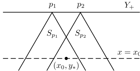
FIGURE 5. Setup for the proof of u_{\partial} \in C^{0,\epsilon}(Y_+) : Shown are the backward light cones from two nearby points p_1, p_2 \in Y_+ that intersect within the slice \{x = x_0\} at a point (x_0, y_*) .
