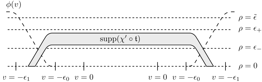
FIGURE 6. Setup for energy estimates near \overline{C_-} : The shaded region is the support of \chi' \circ \mathbf{t} , where -\chi' is used to dominate \chi to give positivity in the energy estimate; near \rho = 0 and on \text{supp}(\chi \circ \mathbf{t}) , i.e. in the region between \rho = 0 and the shaded region, a sufficiently large weight \rho^{-\ell} gives positivity.
