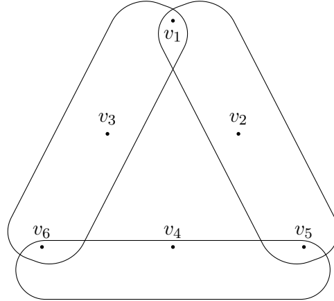
Figure 1: The 3-uniform linear 3-cycle
