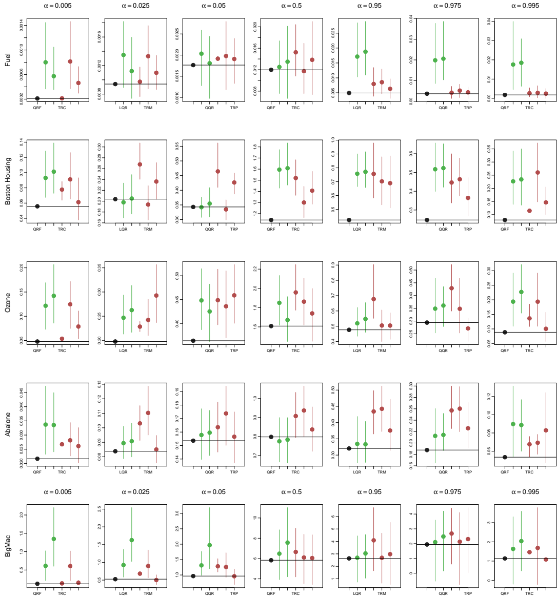
Figure 1: Average loss for various datasets (from top to bottom) and quantiles (from left to right). The average loss of Quantile Regression Forests is shown in each plot as the leftmost dot and is indicated as well by a horizontal line for better comparison. The average losses for competing methods are shown for the linear methods in the middle and the three tree-based methods on the right of each plot. The vertical bars indicate the bootstrap confidence intervals for the difference in average loss for each method against Quantile Regression Forests. Note that no parameters have been fine-tuned for Quantile Regression Forests (the default settings are used throughout).
