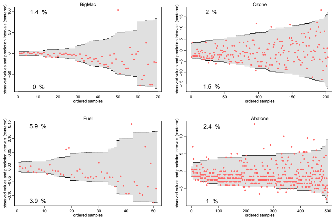
Figure 4: Same plots as in the right panel of Figure 3 for the remaining datasets. Additionally, the percentage of observations that lie above the upper end of their respective prediction intervals (below the lower end) are indicated in the upper left corner (lower left corner). As 95% prediction intervals are shown, on average 2.5% of all observations should be above (and below) their prediction intervals. For the Big Mac, Fuel, and Ozone datasets, it is particularly apparent that the lengths of the prediction intervals vary strongly (some values can thus be predicted more accurately than others).
