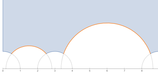
FIGURE 2. The Surface \mathcal{F}_I .
