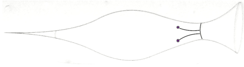
FIGURE 3. The Surface \mathcal{F}_I .
