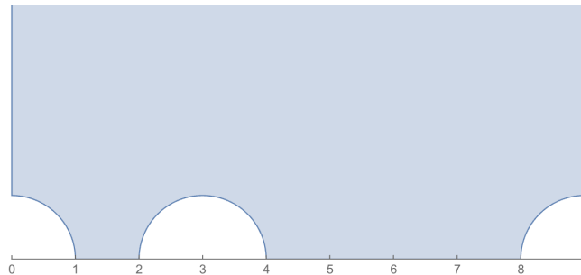
FIGURE 1. Fundamental Domain for \Gamma_I when d = 28 .
