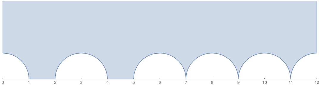
FIGURE 4. Fundamental Domain for \Gamma_J in case d = 28 .
