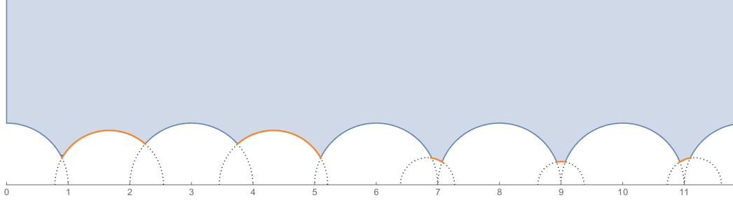
FIGURE 5. The Surface \mathcal{F}_J .
