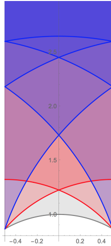
FIGURE 6. Projection of \mathcal{F}_I and \partial\mathcal{F}_I to the modular surface.
