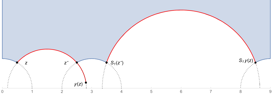
FIGURE 7. Cutting up \partial\mathcal{F}_A .
