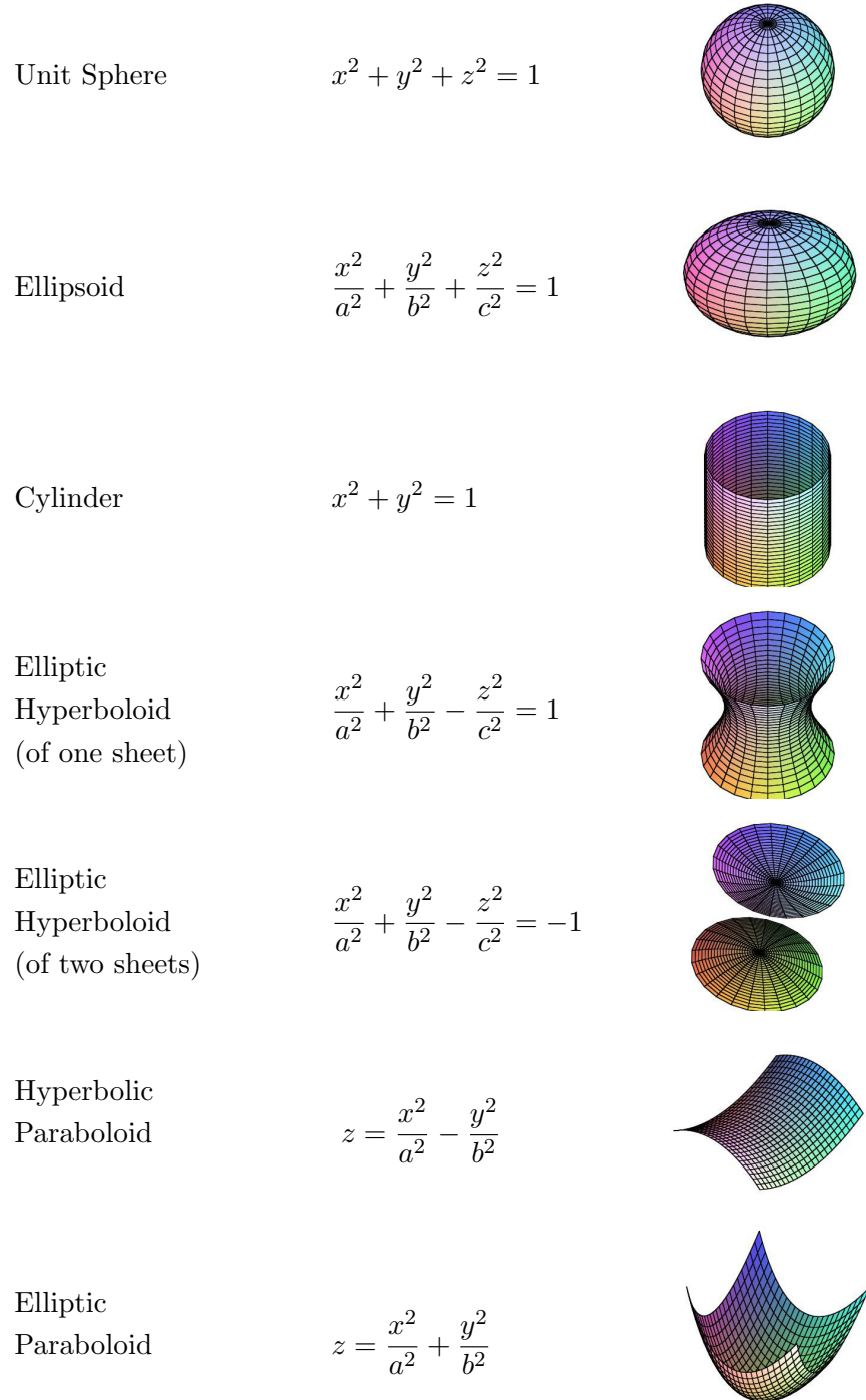
Figure 1.3: Quadric Surfaces.
