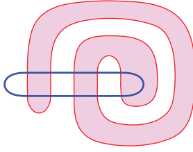
FIGURE 13. Four primitive lunes in the 2-sphere.
