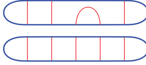
FIGURE 12. \alpha encircles at least two primitive lunes.
