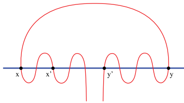
FIGURE 27. Lunes from x or x' to y or y' .
