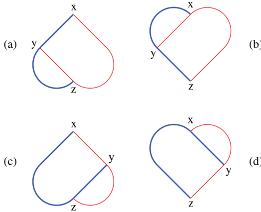
FIGURE 23. Four broken hearts.
