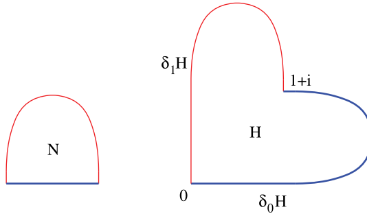
FIGURE 24. The domains N and H .
