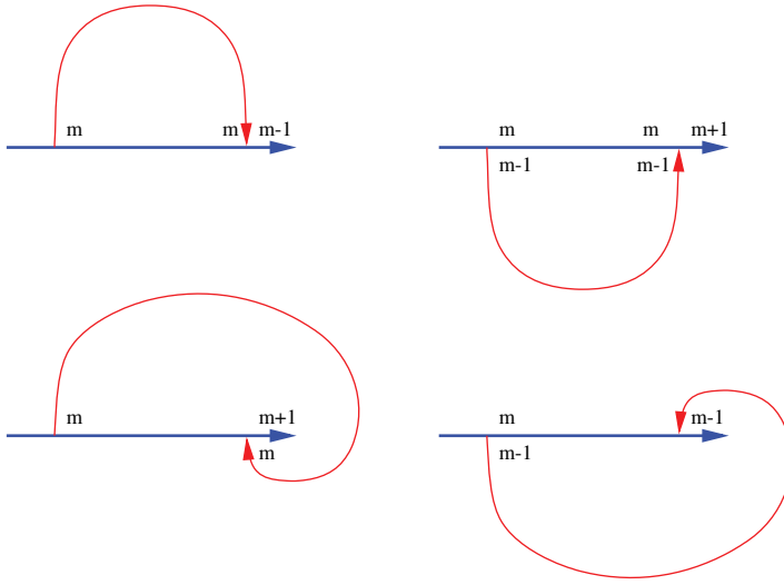
FIGURE 15. Simple arcs.
