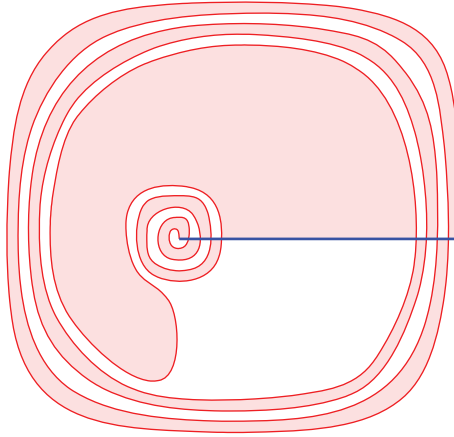
FIGURE 20. A lune of large area.
