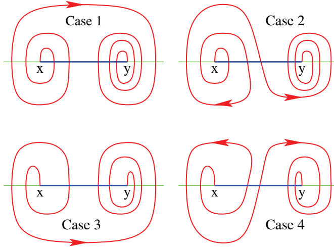
FIGURE 4. Reduced (\alpha, \beta) -traces in \mathbb{C} .
