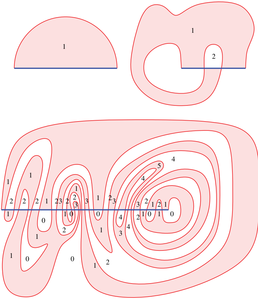
FIGURE 9. Three lunes.
